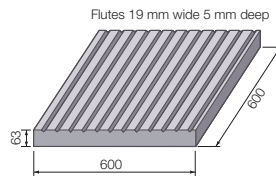
Fluted paving
