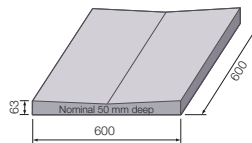
Dished paving
